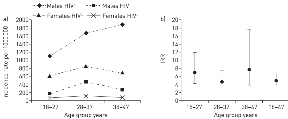
FIGURE 1 a) Incidence rate of confirmed tuberculosis (TB) among the HIV-infected and -uninfected population of the district of Manhiça, Mozambique in 2011. b) Incidence rate ratio (IRR) of TB among the HIV-infected population compared with the HIV-uninfected population by age group in the district of Manhiça in 2011. Whiskers represent 95% confidence intervals.
