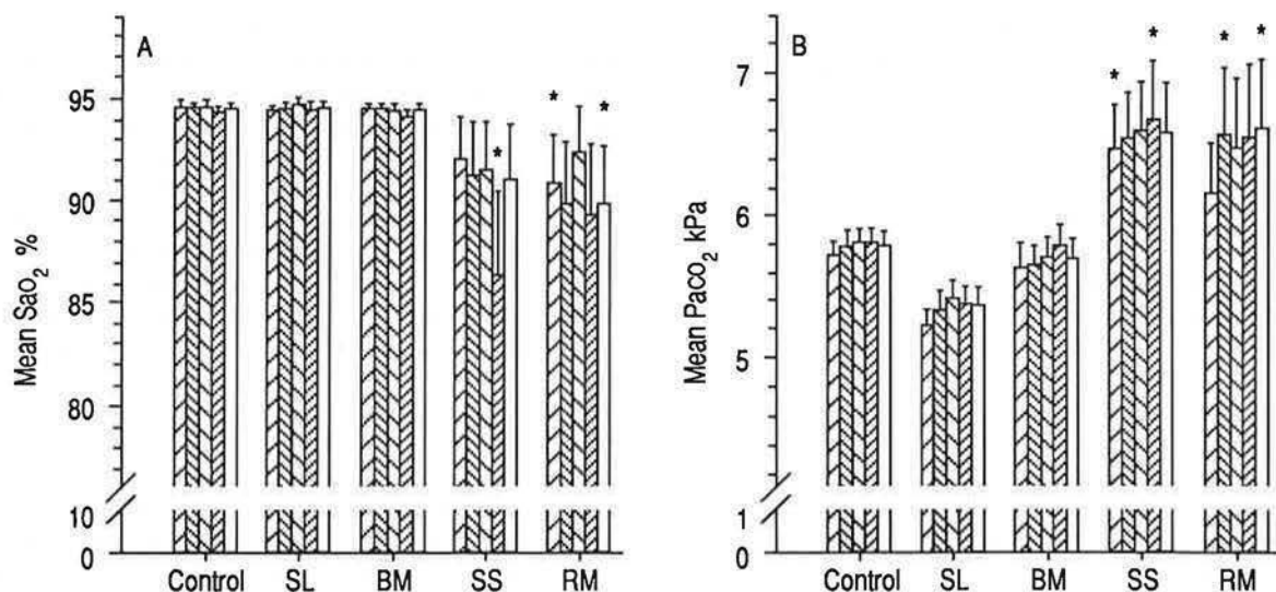
Fig. 1. — A) mean arterial saturation ( \text{Sao}_2 ); and B) mean arterial carbon dioxide tension ( \text{Paco}_2 ) with standard error for the control group, as well as the spinal limb (SL), bulbar muscle (BM), spinal scoliotic (SS) and respiratory muscle (RM) polio groups. \square : Stage 1 sleep; \square : Stage 2 sleep; \square : slow wave sleep; \square : rapid eye movement sleep; \square : total time asleep. *: significantly different from control group ( p < 0.05 ).
