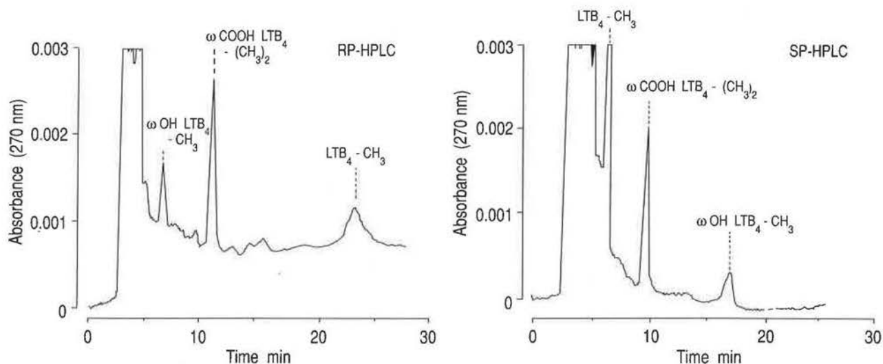
Fig. 1. - Analysis of leukotrienes extracted from the bronchoalveolar lavage fluid of patient No. 6 (table 1a) after methacholine challenge. In addition to the conventional RP-HPLC system, LTB_4 and its omega-oxidation products ( \omega OH- LTB_4 and \omega COOH- LTB_4 ) are separated as methylated derivatives isocratically (SP-HPLC) and with gradient-elution (RP-HPLC). RP-HPLC: reverse-phase high pressure liquid chromatography (HPLC); SP-HPLC: solid-phase HPLC; LTB_4 : leukotriene B_4 .
