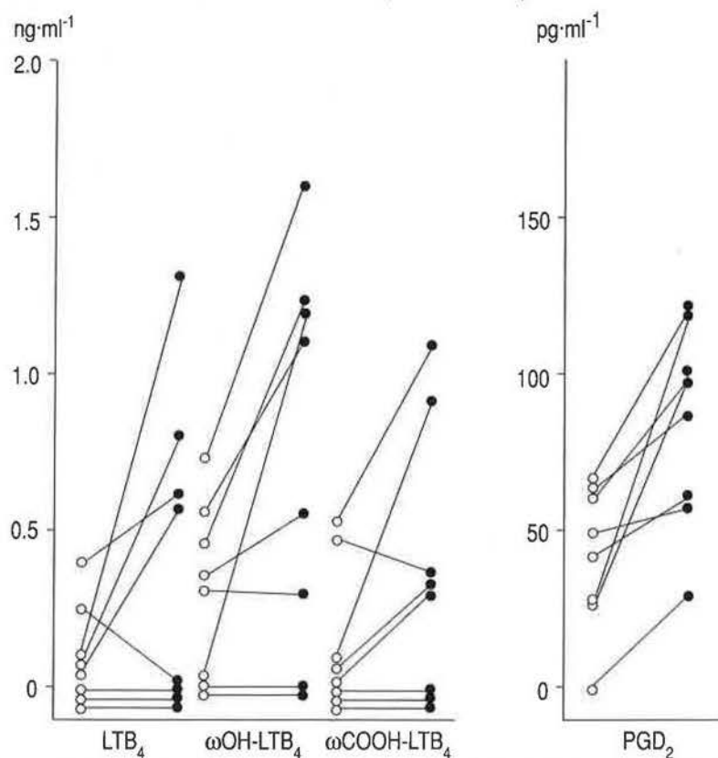
Fig. 2. - Bronchoalveolar lavage leukotriene B_4 and its omega oxidation products ( LTB_4 , \omega OH- LTB_4 and \omega COOH- LTB_4 ) and prostaglandin D_2 ( PGD_2 ) levels in asthmatic patients without (open circles) and 5 h after methacholine challenge (closed circles).
